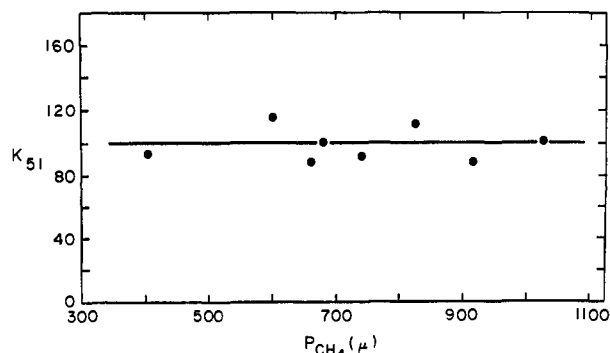
Figure 5. Equilibrium constant vs. \text{CH}_4 pressure for \text{H}_3\text{O}\cdot\text{CH}_4^+ + \text{CH}_4 \rightleftharpoons \text{H}_3\text{O}\cdot(\text{CH}_4)_2^+ . P_{\text{H}_2\text{O}} = 0.35 \mu , T = -60^\circ .
