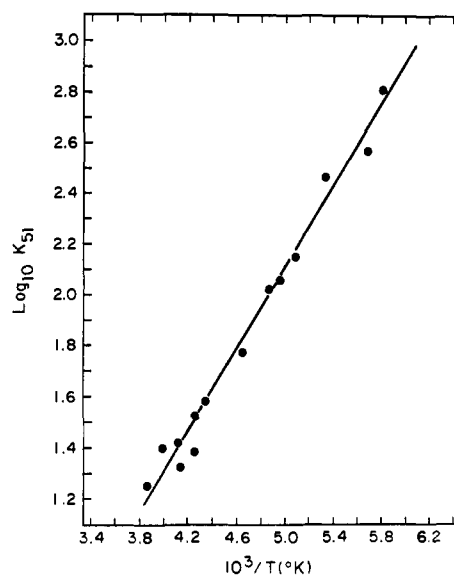
Figure 6. Van't Hoff plot for \text{H}_3\text{O}\cdot\text{CH}_4^+ + \text{CH}_4 \rightleftharpoons \text{H}_3\text{O}\cdot(\text{CH}_4)_2^+ . Standard state = 1 atm, P_{\text{CH}_4} = 900 \mu , P_{\text{H}_2\text{O}} = 0.40 - 0.30 \mu .
