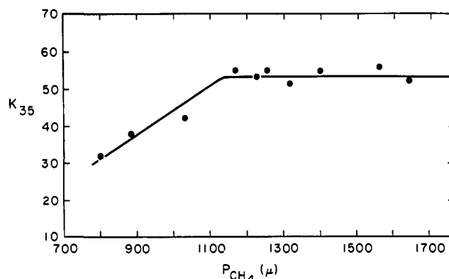
Figure 1. Equilibrium constant vs. CH 4 pressure for H 3 O + + CH 4 ⇌ H 3 O·CH 4 + . P_{\text{H}_2\text{O}} = 0.5 \mu , T = 28^\circ .
